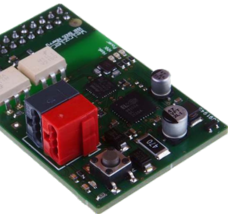
BAOS Development Kit (Art.-No. 5240)
